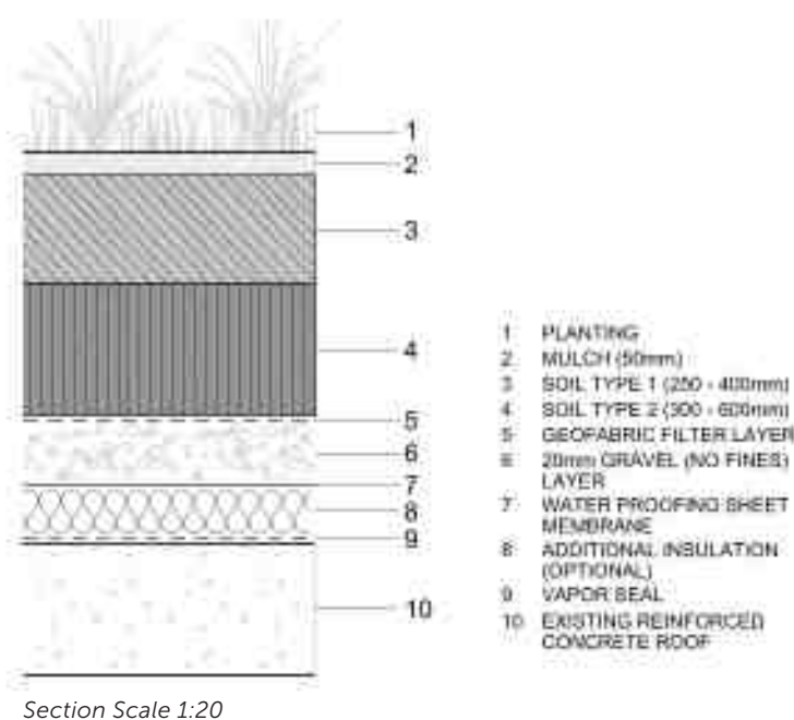
Intensive green roof typical detail
