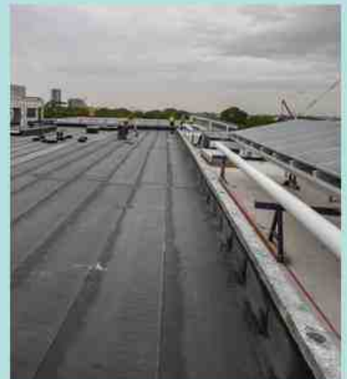
Waterproofing on the Yerrabingin green roof, South Eveleigh
