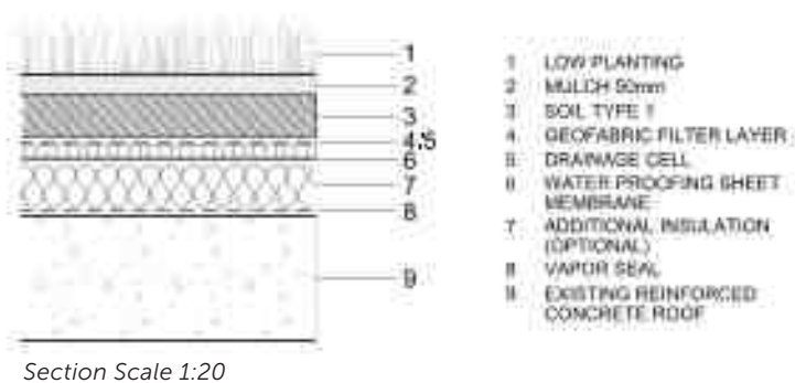
Extensive green roof typical detail
