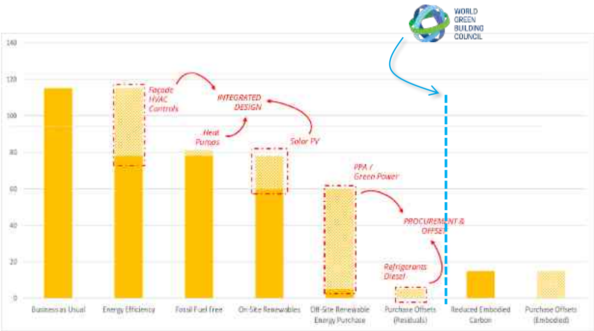
Pathway to Net Zero Emissions
