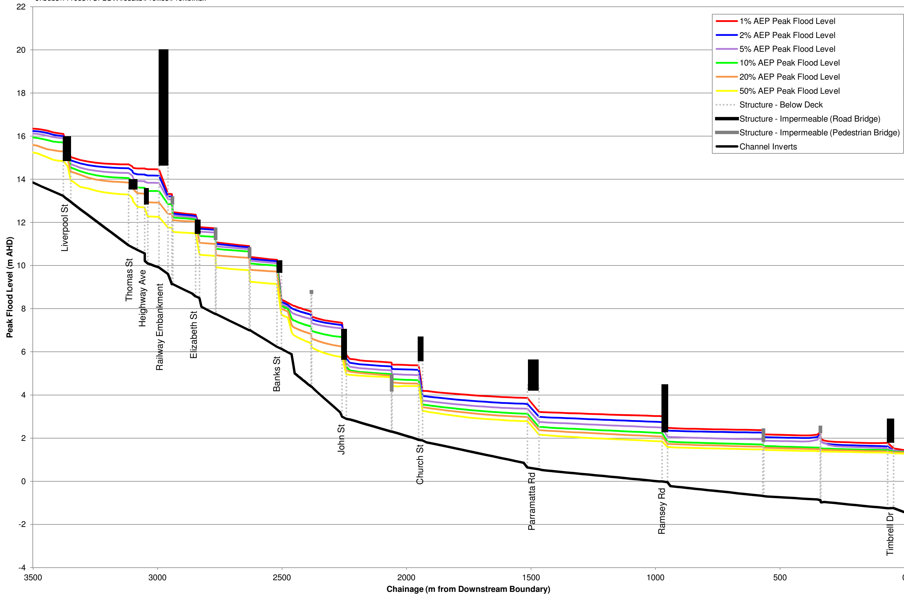
FIGURE 11A PEAK FLOOD LEVEL PROFILES DESIGN EVENTS
