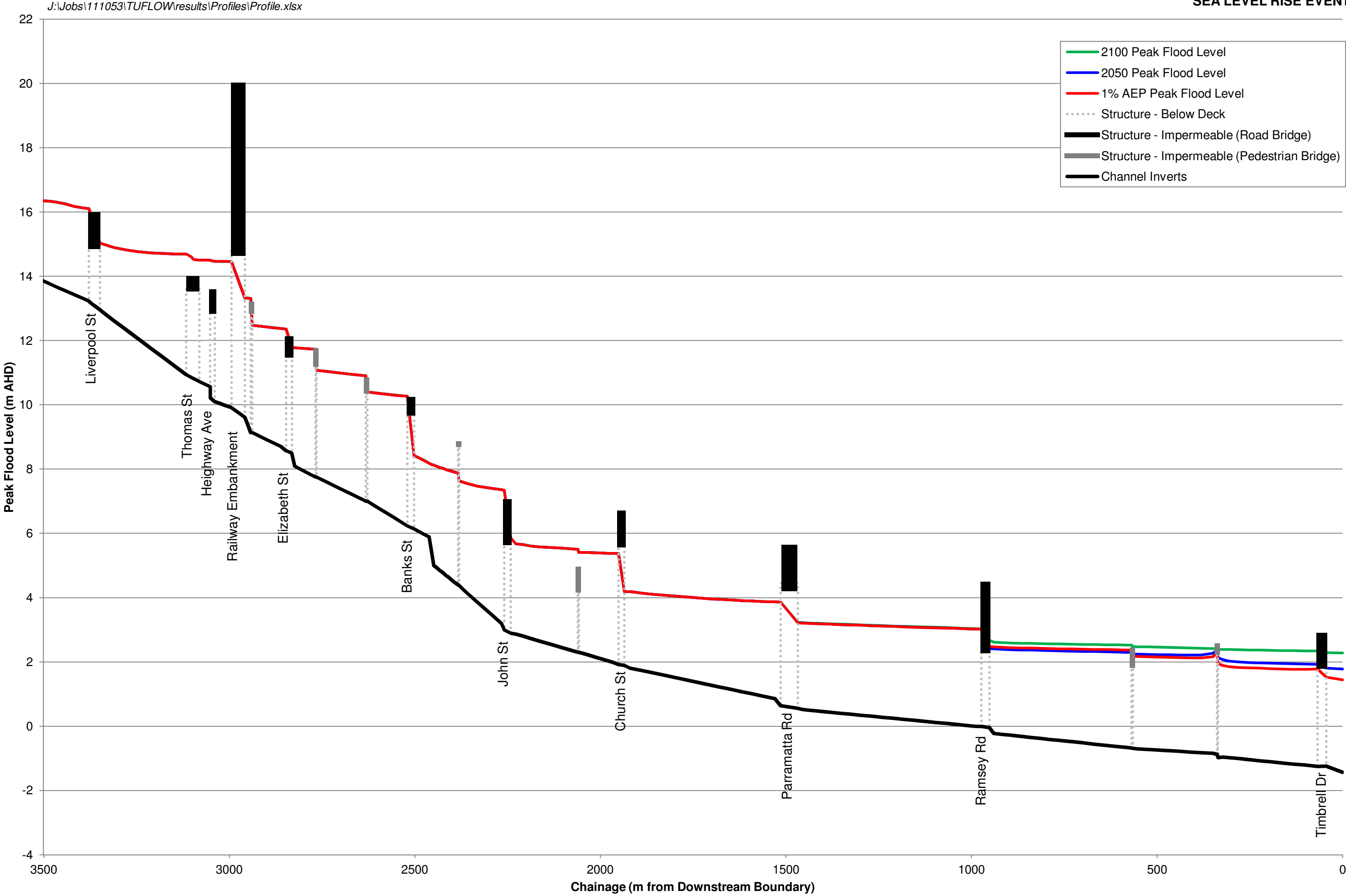
FIGURE 11B PEAK FLOOD LEVEL PROFILES SEA LEVEL RISE EVENTS
