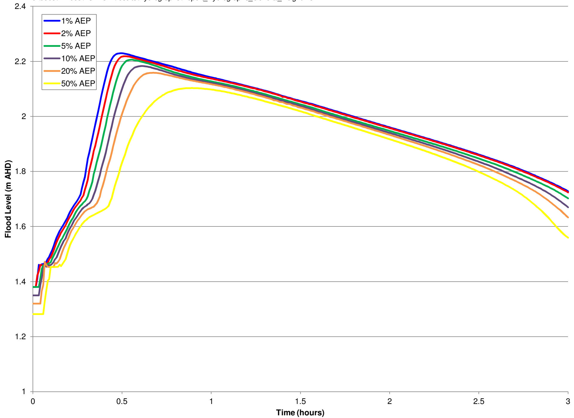
FIGURE 12A DESIGN FLOOD LEVEL HYDROGRAPH DOBROYD PARADE
