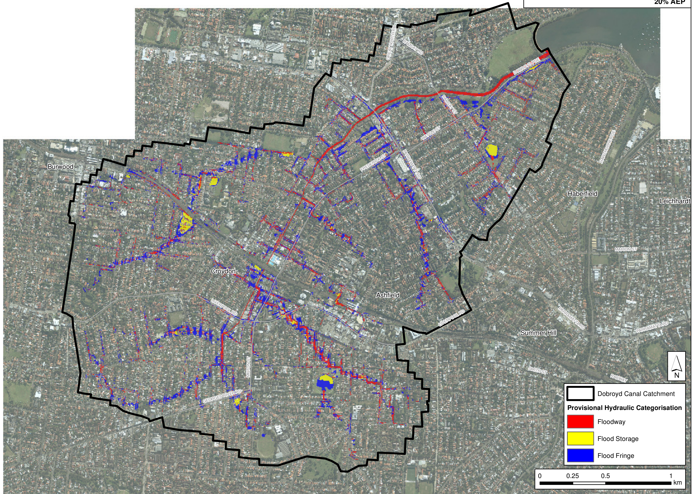
FIGURE 25 PROVISIONAL HYDRAULIC CATEGORISATION 20% AEP
