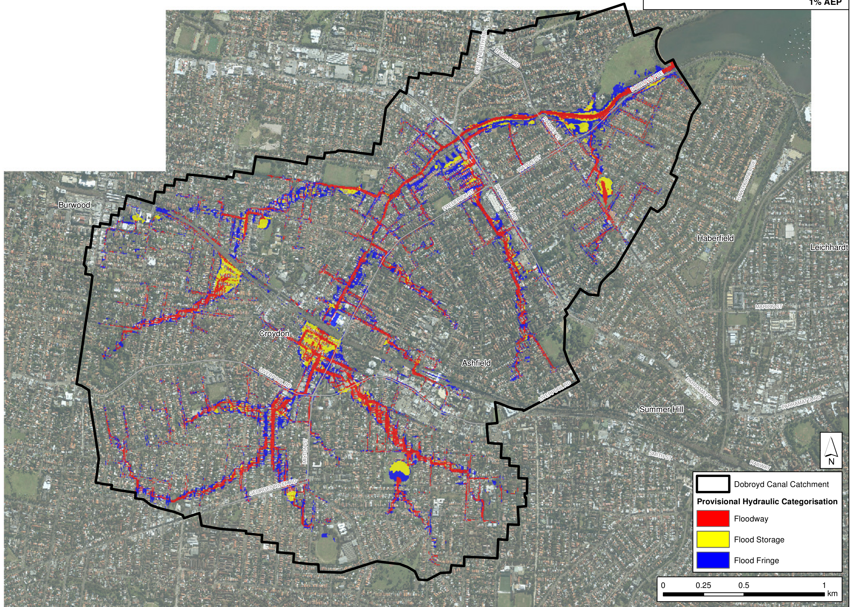
FIGURE 27 PROVISIONAL HYDRAULIC CATEGORISATION 1% AEP
