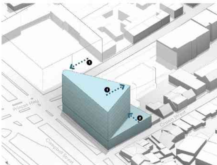
Figure 6-3: Drawing showing orientation of tower set back to maximise solar gain and minimise overshadowing and continue adjacent street grid. Source: Scott Carver 2023
