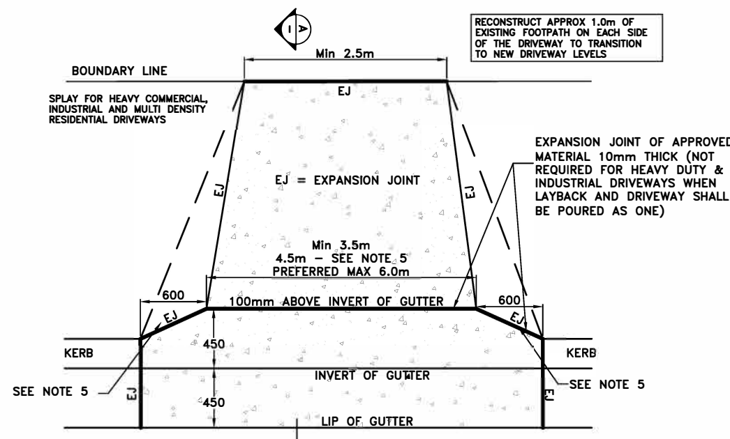
DRIVEWAY SPECIFICATION-'A' (FULLY PAVED FOOTPATH) (ORIGINAL = A3 SHEET) NOT TO SCALE
