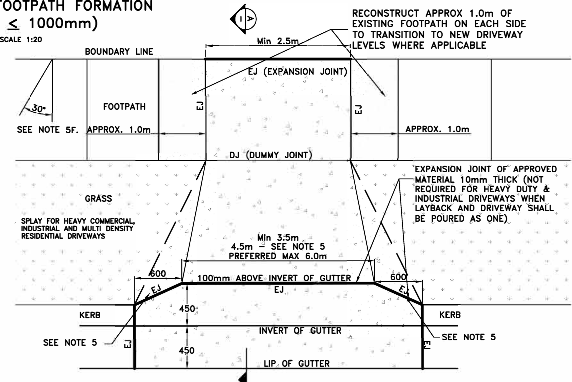
DRIVEWAY SPECIFICATION-'B' WITH GRASS VERGE NOT TO SCALE
