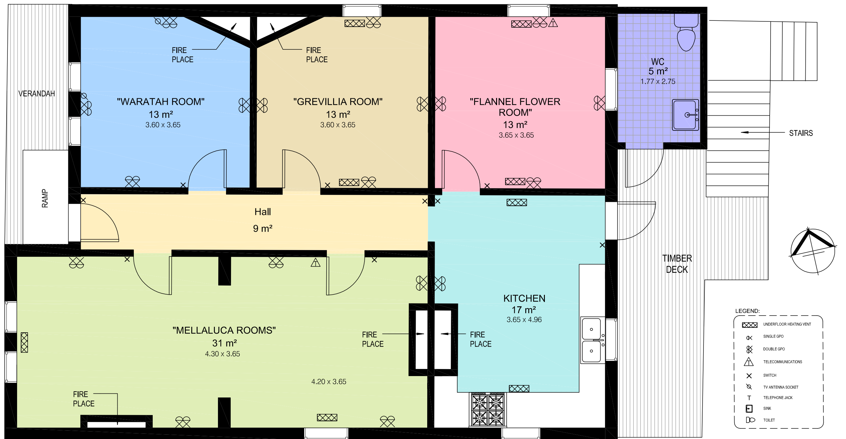
GROUND FLOOR PLAN "WHITES CREEK COTTAGE"
