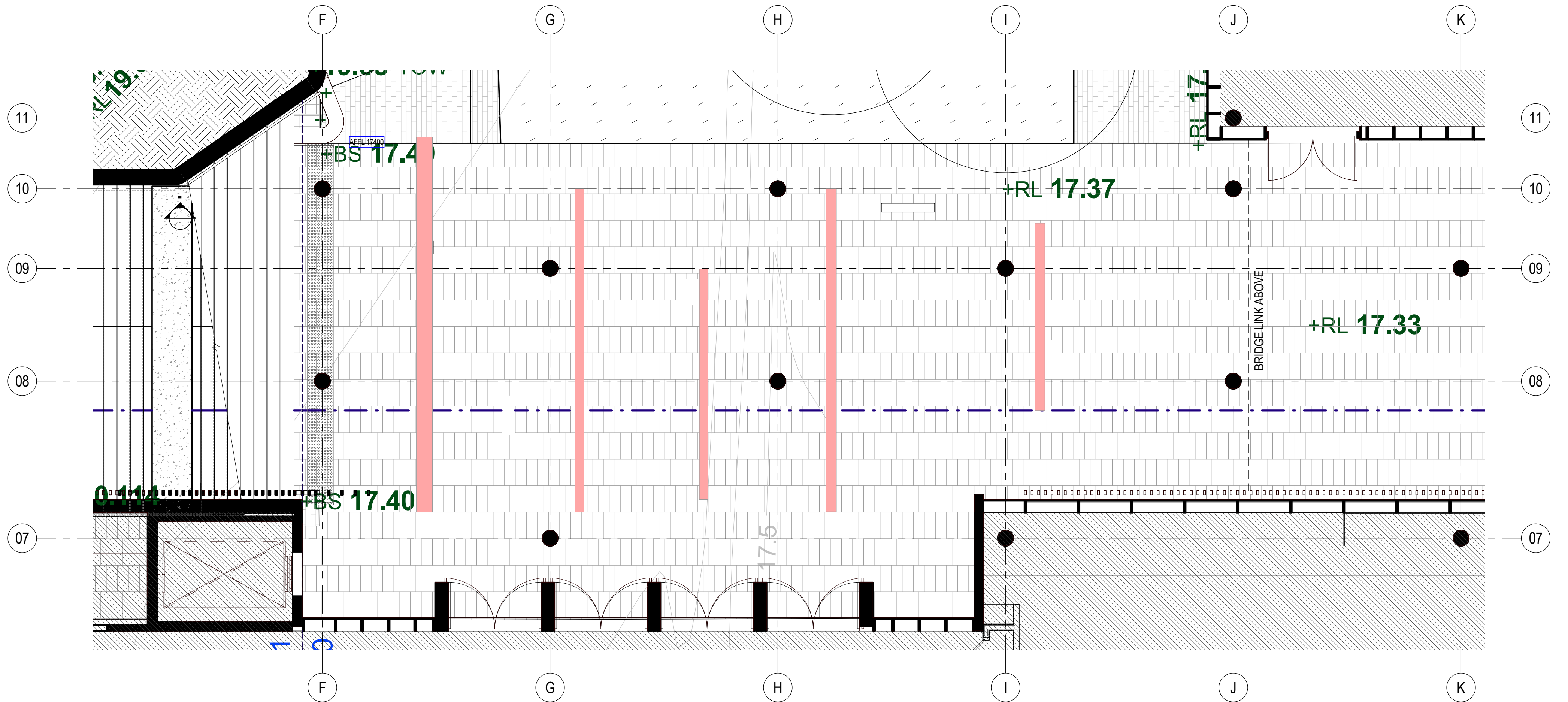
1 LEVEL 00 - ENTRY PAVING OPENINGS D-XX-01 1:50
