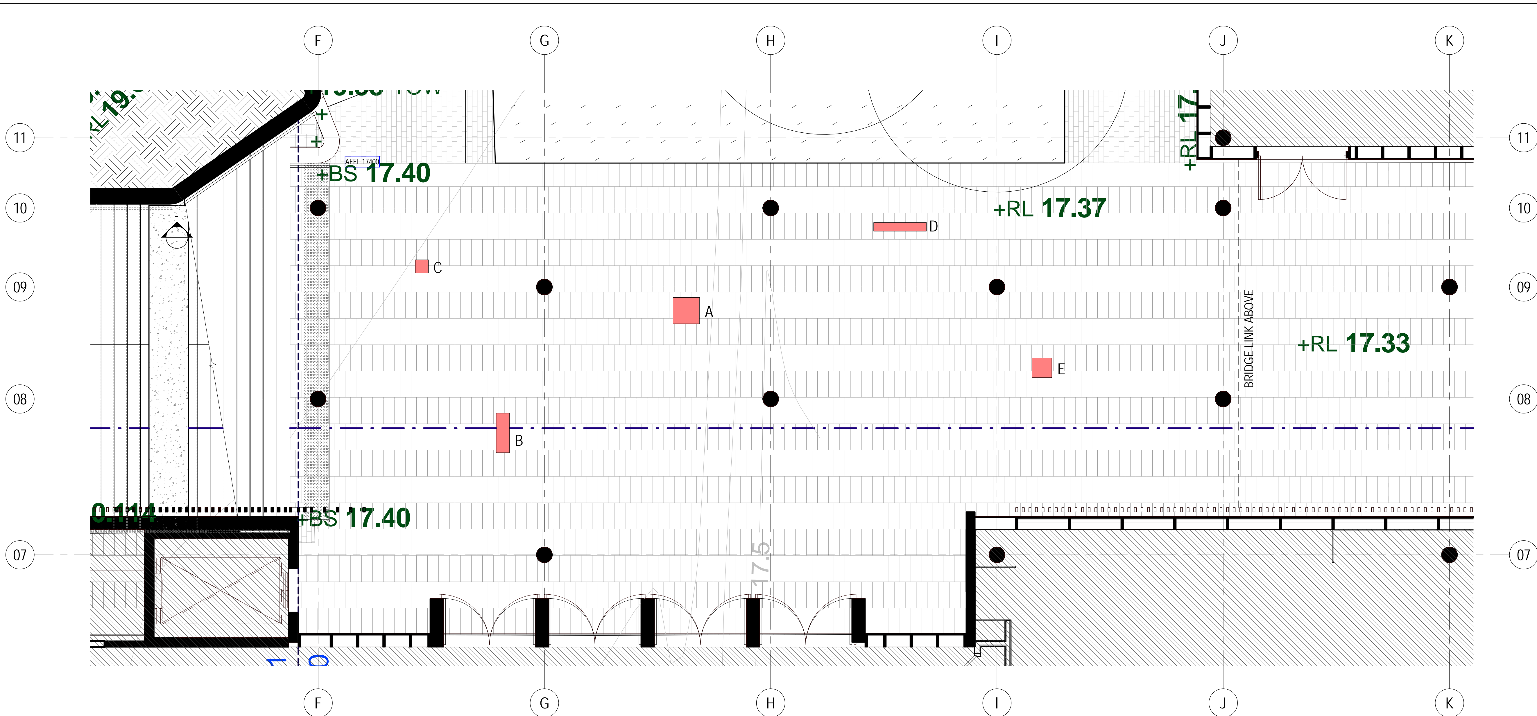
1 LEVEL 00 - ENTRY PAVING OPENINGS D-XX-01 1:50
