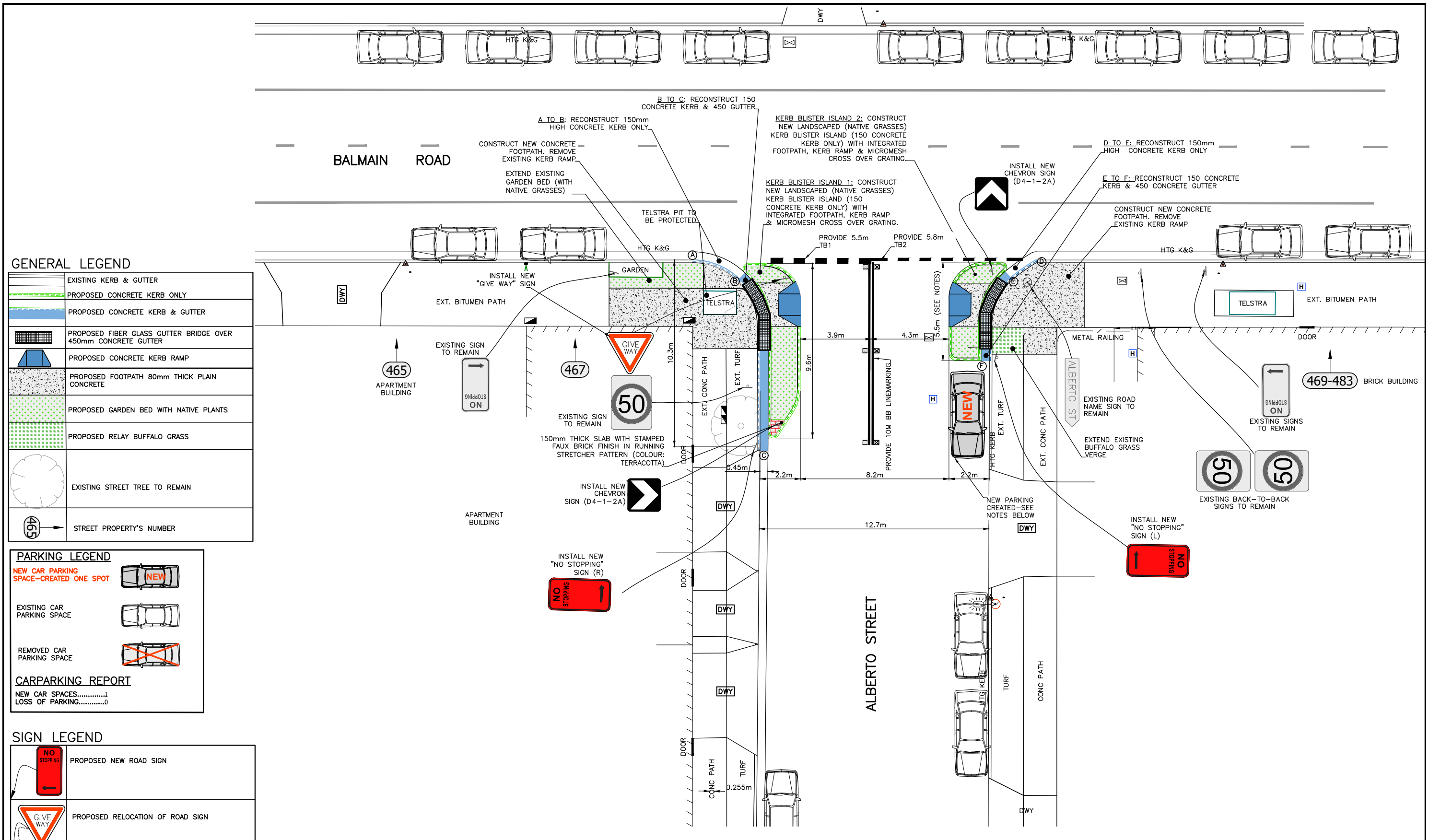
PLAN VIEW SCALE 1:100 (A1 PLOT)
